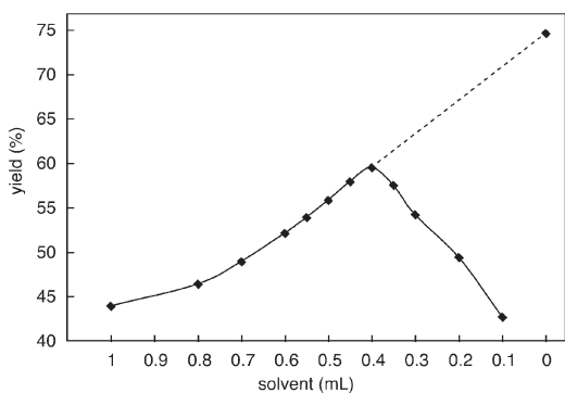
Fig. 1 Concentration effect: Yields of Wittig reaction of 1f with 4a in HCSM after 5 min.
